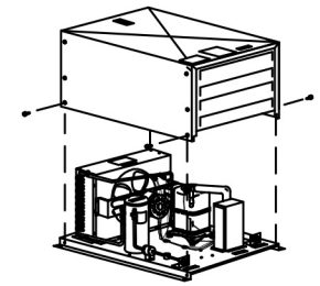
CONDENSING UNIT DETAIL
