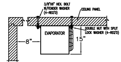
EVAPORATOR MOUNTING DETAIL
