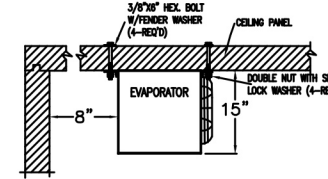
EVAPORATOR MOUNTING DETAIL
