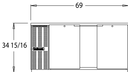
BBUC69S FRONT VIEW
