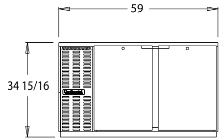
BBUC59S FRONT VIEW
