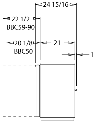
BBUC50,59,69,79 & 90 SHALLOW SIDE VIEW
