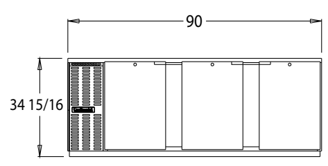
BBUC90S FRONT VIEW
