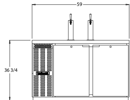
KC59 FRONT VIEW
