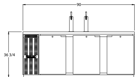
KC90 FRONT VIEW
