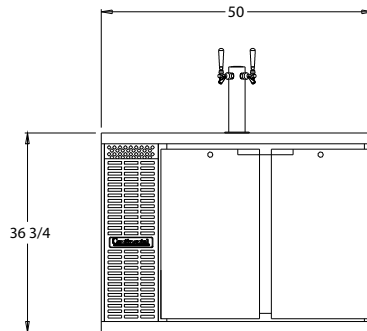
KC50 FRONT VIEW
