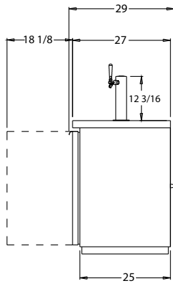
KC50,59,69,79 & 90 SIDE VIEW
