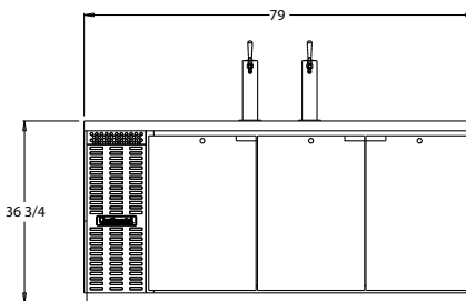
KC79 FRONT VIEW
