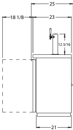
KC50,59,69,79 & 90 SHALLOW SIDE VIEW
