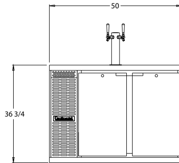
KC50 FRONT VIEW
