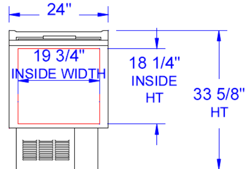
FRONT GF24L
