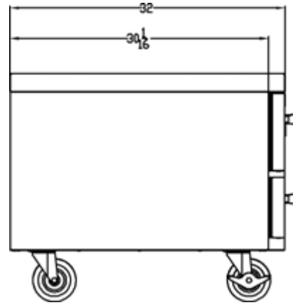
END VIEW
