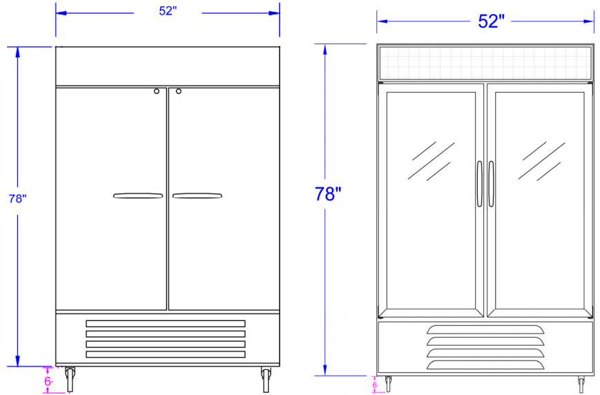
FRONT HBRF49-1-G FRONT
