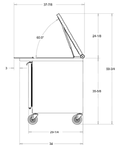
SPE60-24M-STL END VIEW WITH LID OPEN
