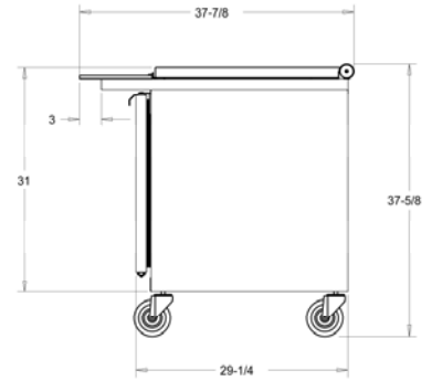
SPE60-24M-STL END VIEW WITH LID CLOSED
