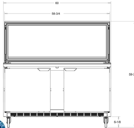
SPE60-24M-STL FRONT VIEW WITH LID CLOSED
