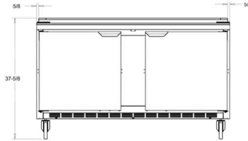
SPE60-24M-STL FRONT VIEW WITH LID CLOSED
