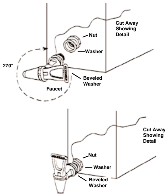
Fig. 1 Premium Faucet: 10850, 10854, 10851, 10855
