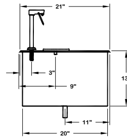
ELEVATION VIEW
