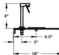
SECTIONAL VIEW
