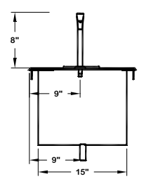
SECTIONAL VIEW
