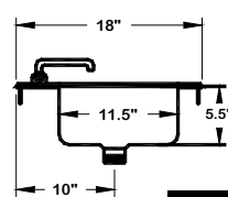
SECTIONAL VIEW
