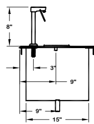
SECTIONAL VIEW
