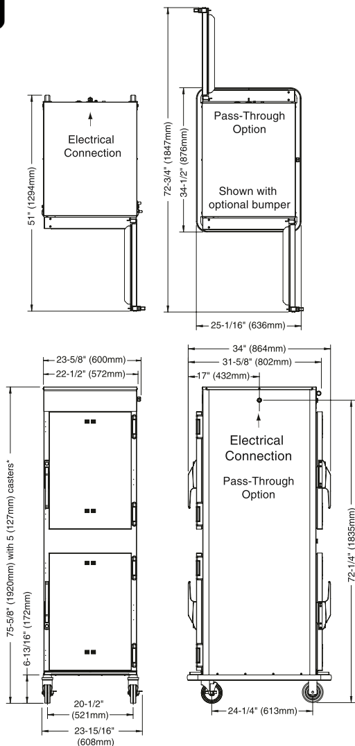
*73-7/8" (1877mm) - with optional 3-1/2" casters *74-11/16" (1897mm) - with optional 6" legs
