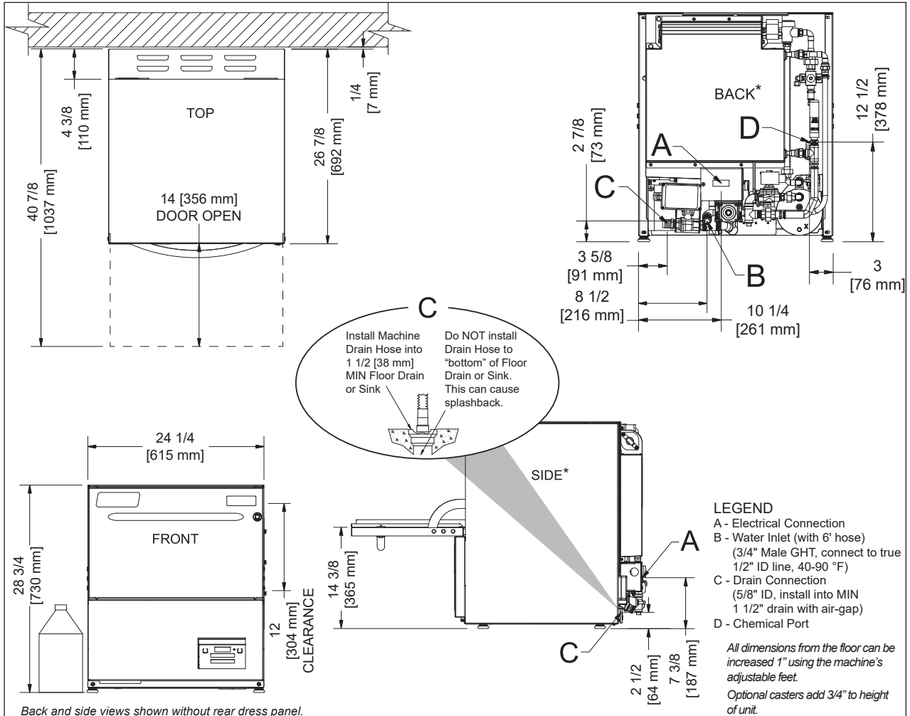
Back and side views shown without rear dress panel.
