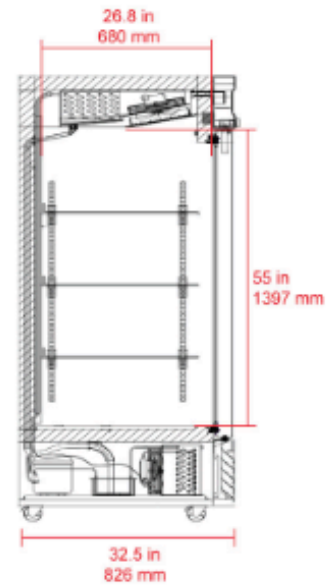
SIDE VIEW (ALL MODELS)
