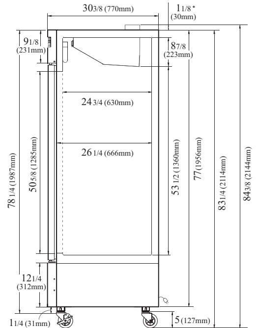
SIDE VIEW *Pressure relief valve
