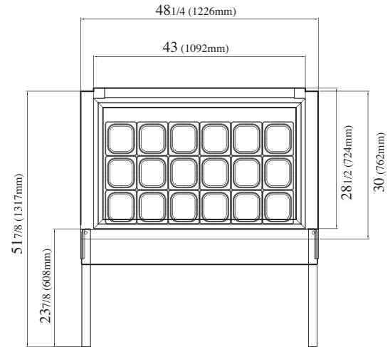
PLAN VIEW
