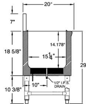
w/ 10-Circuit Cold Plate (-XD Model Shown)
