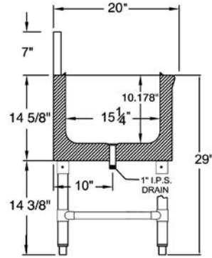
Non-Cold Plate
