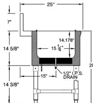
w/ 10-Circuit Cold Plate
