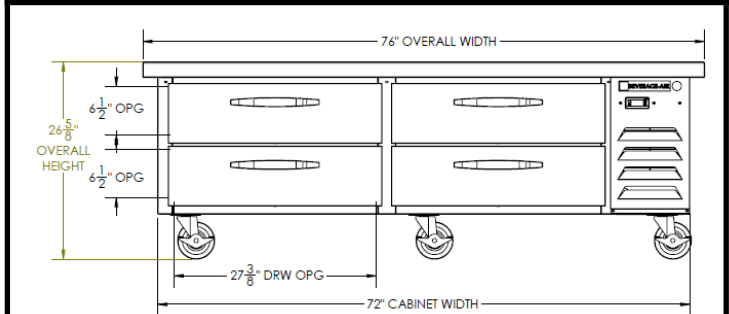
Elevation View
