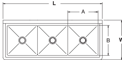
3 COMP - 1 DRBD
