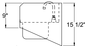
WH-14-S SIDE VIEW
