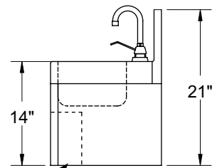
PAPER TOWEL DISPENSER WDH-14 SIDE VIEW
