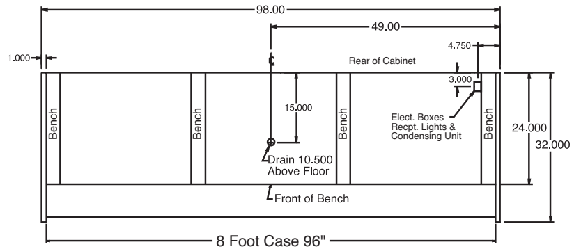
Plan Views
