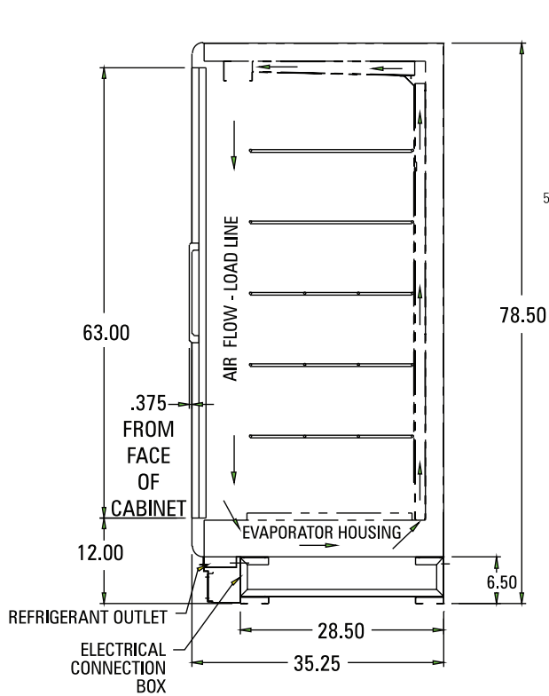
Cross Section
