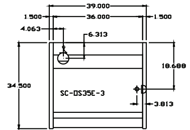
3' Plan View
