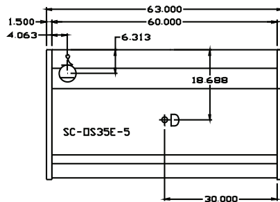
5' Plan View
