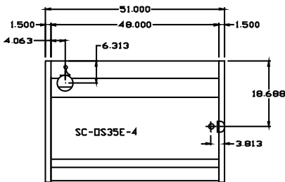
4' Plan View
